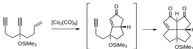
Scheme 13. Synthesis of a fenestrene by domino-Pauson–Khand reaction according to Keese.
