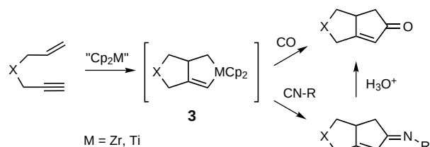
Scheme 5. Metallocene-mediated Pauson–Khand type reactions.
