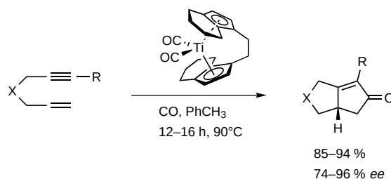
Scheme 6. Catalytic enantioselective bicyclizations according to Buchwald.
