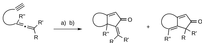
Scheme 8. Pauson–Khand reactions with allenes. a) [\text{Co}_2(\text{CO})_8] ; b) 6 equiv of N -methylmorpholin- N -oxide, THF/ \text{CH}_2\text{Cl}_2 , -78 \rightarrow 20^\circ\text{C} , 3 h.
